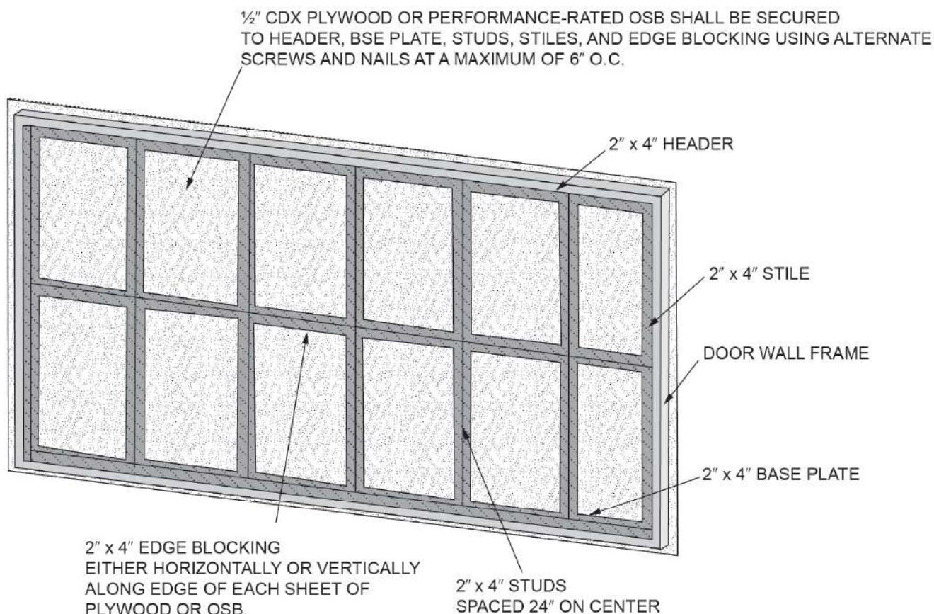
FIGURE A103.1(2) BOARDING OF DOOR WALL
